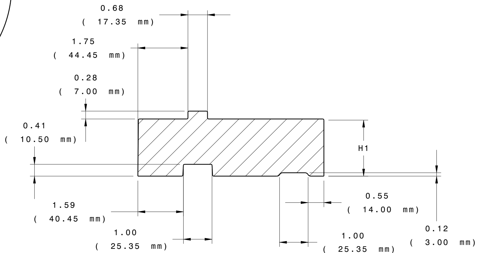
Section cut A-A
